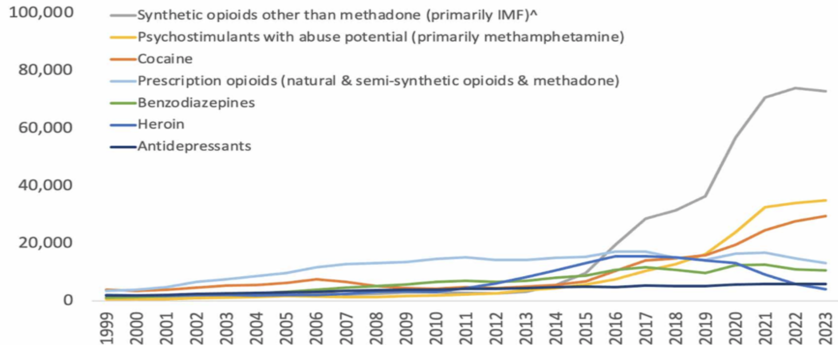
Figure 2. U.S. Overdose Deaths*, Select Drugs or Drug Categories, 1999-2023
